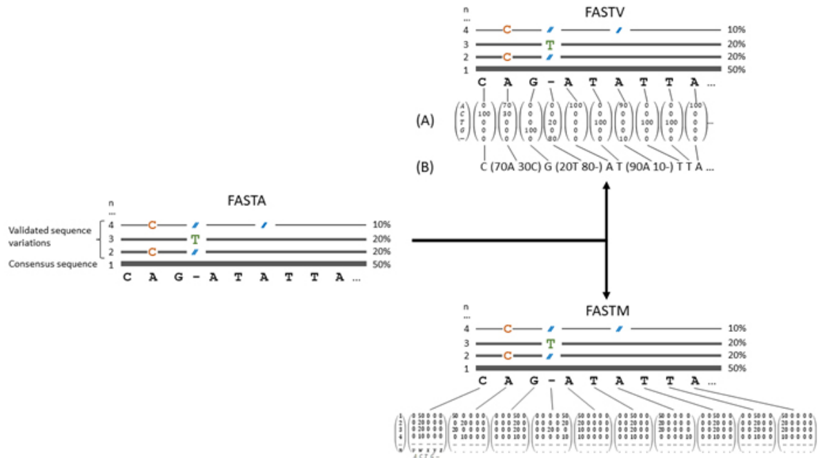
Figure 2. Potential FASTA successor formats FASTV and FASTM. For FASTV, each genome position is depicted either by a matrix “()” (FASTV A) or a human readable notation (FASTV B), where a single genome location comprises the normalised distribution value of one of the four bases or a gap, ignoring bases that do not occur at this position. In FASTV, the frequency of nucleotides per position is captured but not their respective occurrences across subpopulations. For FASTM, a two-dimensional matrix enables capturing not only the relative distribution of nucleotide variations for every genome position, but the matrix further enables the tracking of individual subpopulations.
