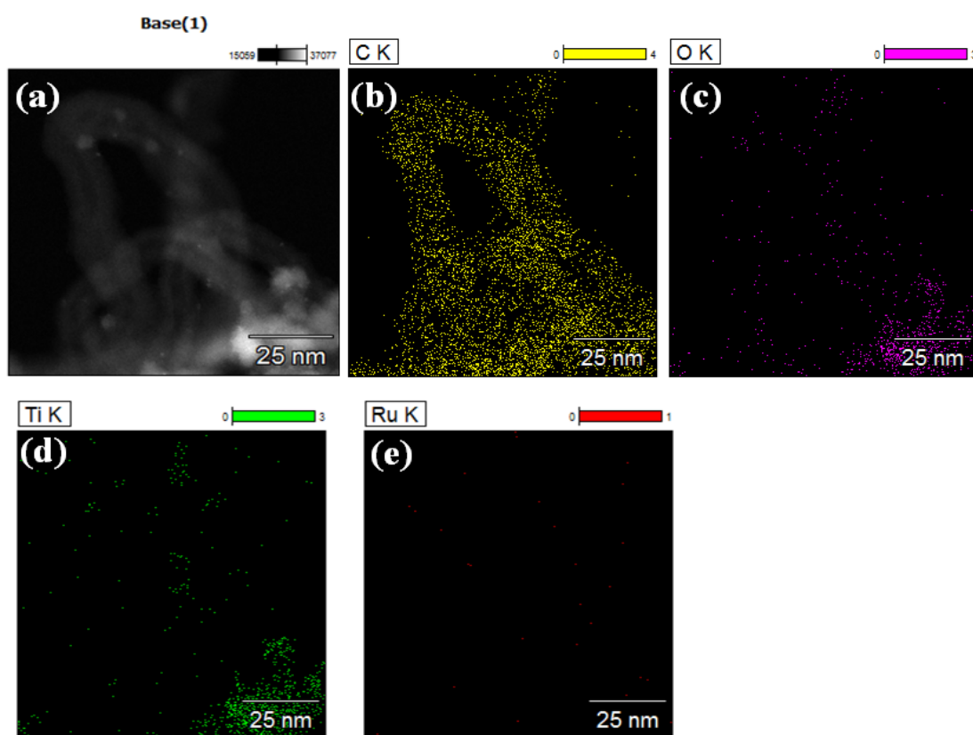
Figure S1. HR-TEM EDS mapping of Ru/TiO 2 /CNTs.
