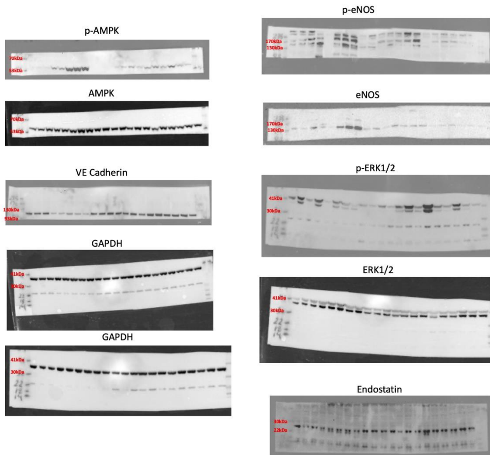
Supplemental Figure 1: Complete immunoblots. p-, phosphorylated; AMPK 5' adenosine monophosphate-activated protein kinase (AMPK); p-, phosphorylated; ERK1/2, extracellular signal-regulated kinase 1/2; eNOS, endothelial nitric oxide synthase; VE-Cadherin, vascular endothelial cadherin; GAPDH, glyceraldehyde 3-phosphate dehydrogenase.
