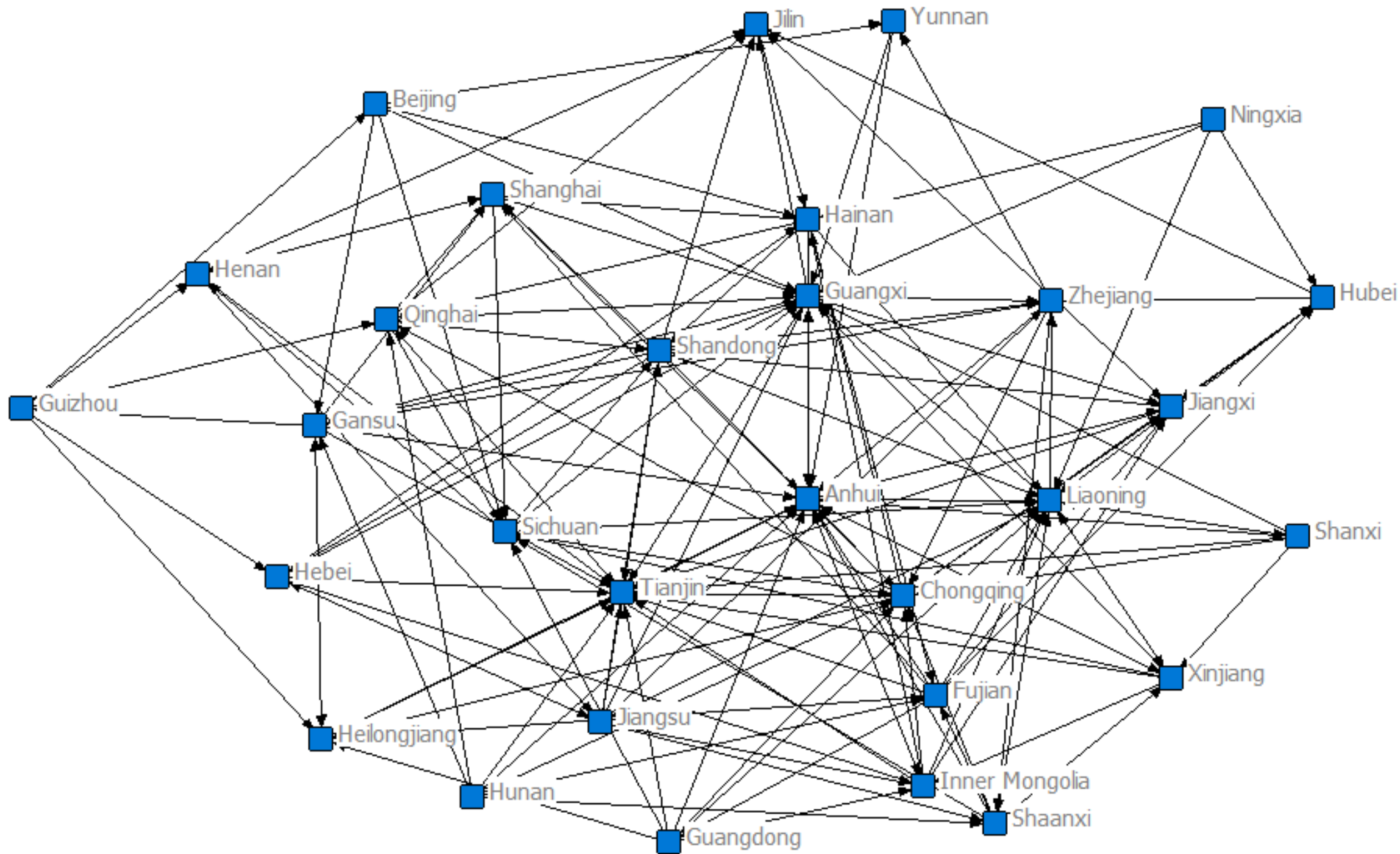
Carbon emission footprint spatial network in 2010
