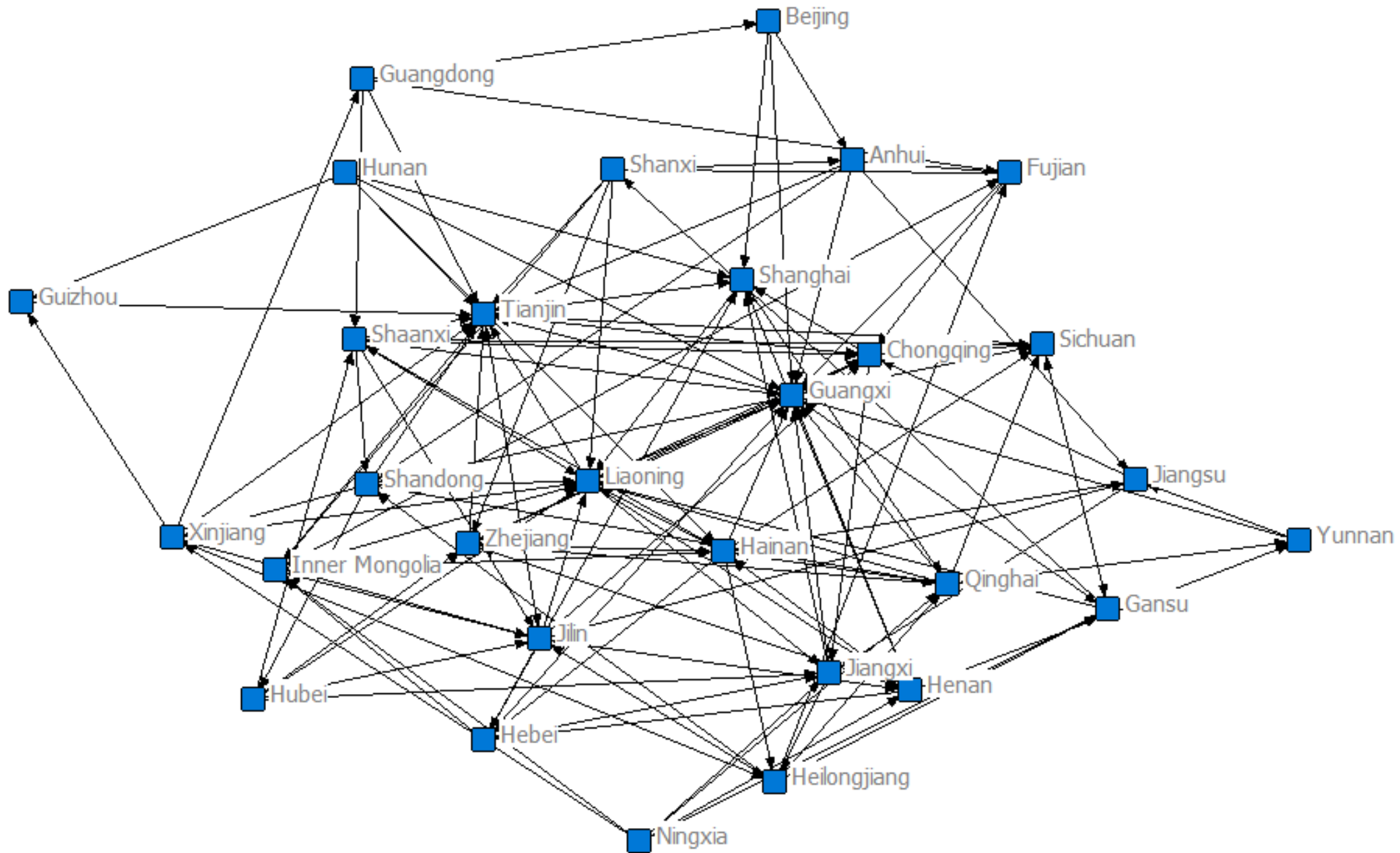
Carbon emission footprint spatial network in 2011
