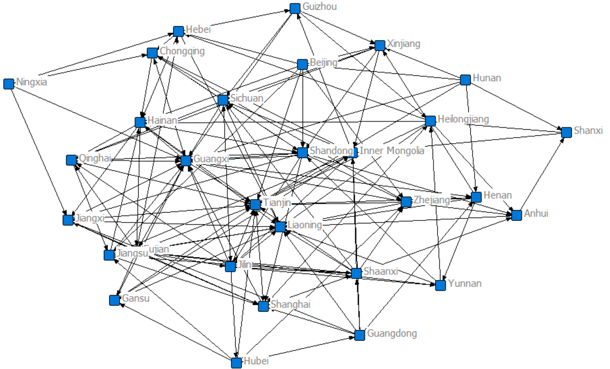
Carbon emission footprint spatial network in 2020
