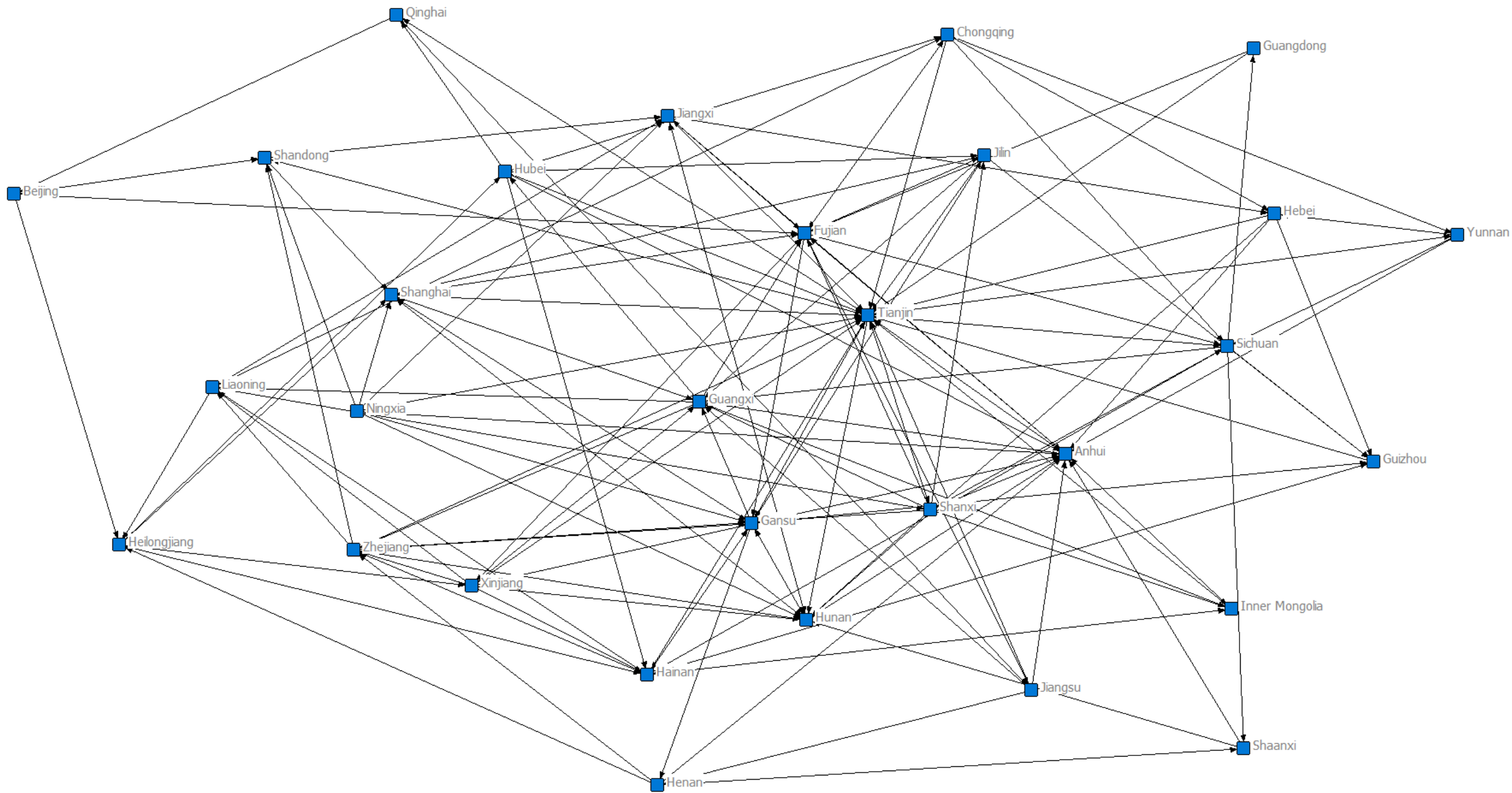
Carbon emission footprint spatial network in 2005
