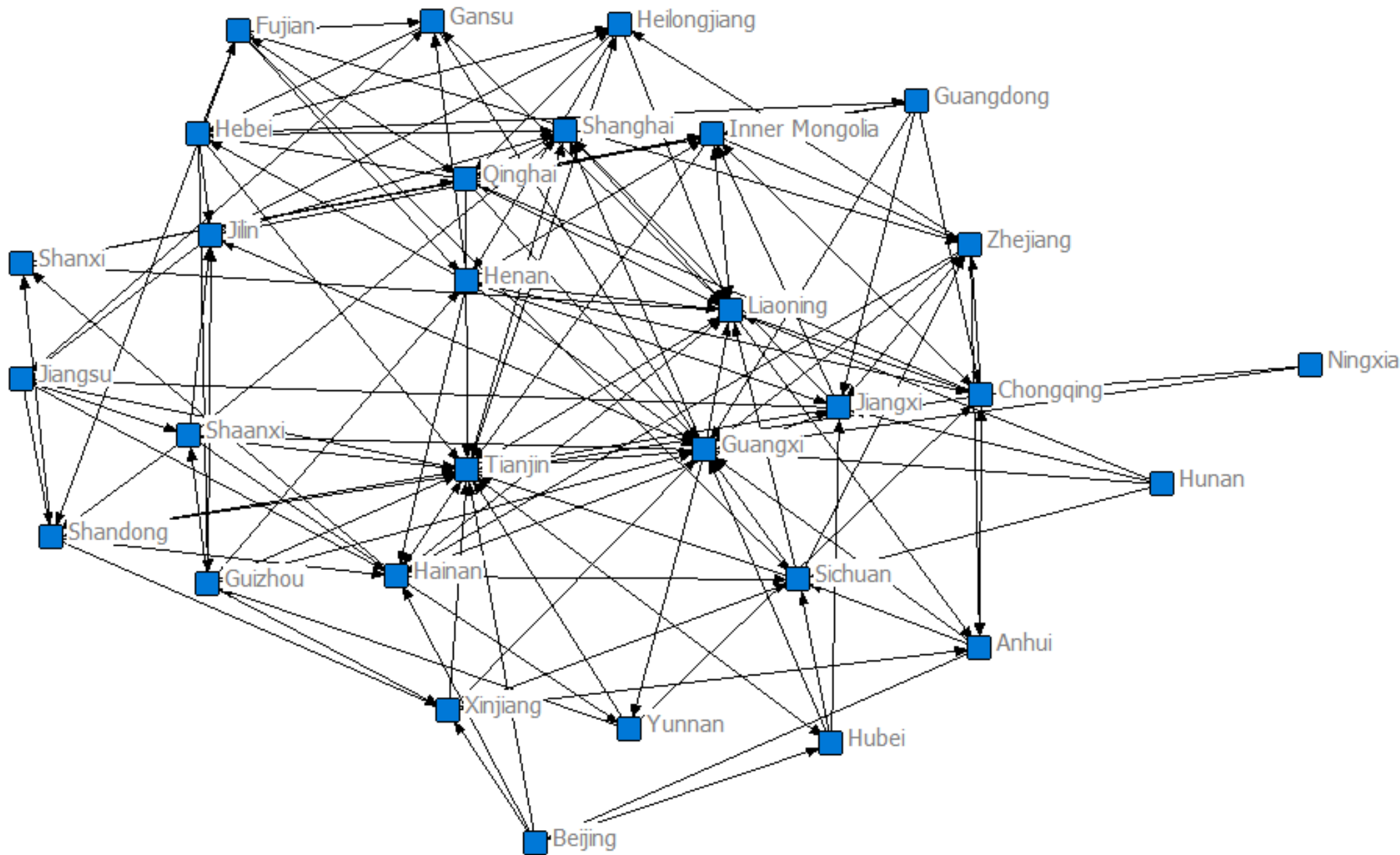
Carbon emission footprint spatial network in 2012
