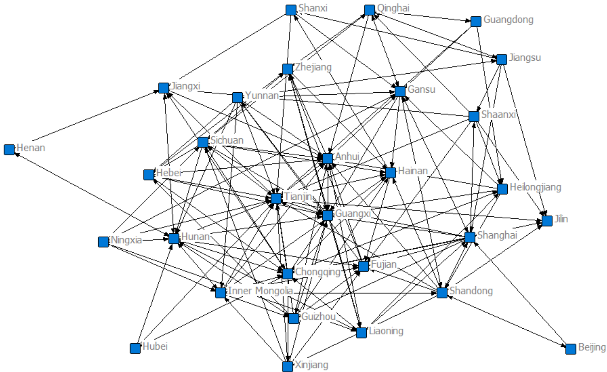
Carbon emission footprint spatial network in 2008
