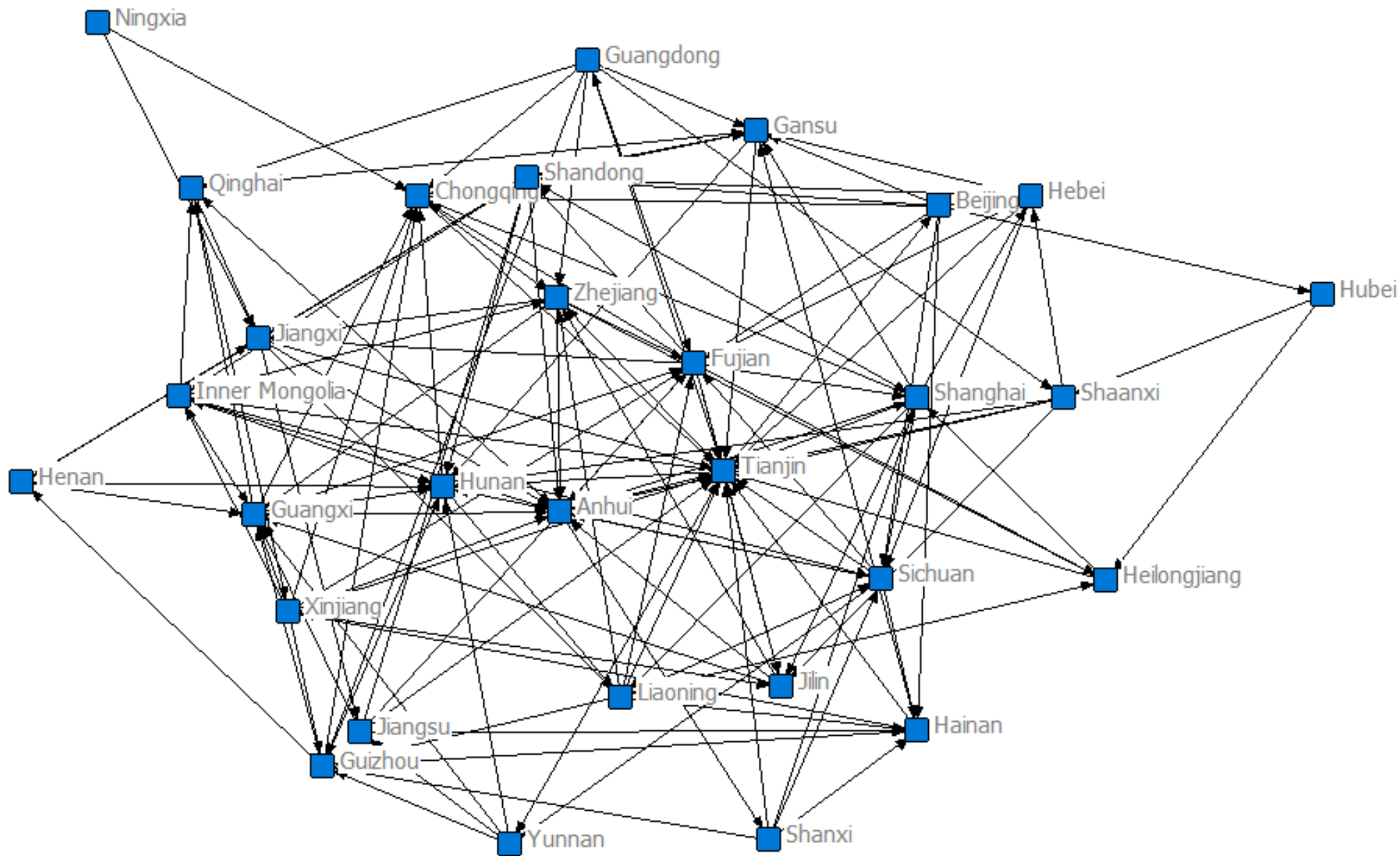
Carbon emission footprint spatial network in 2006
