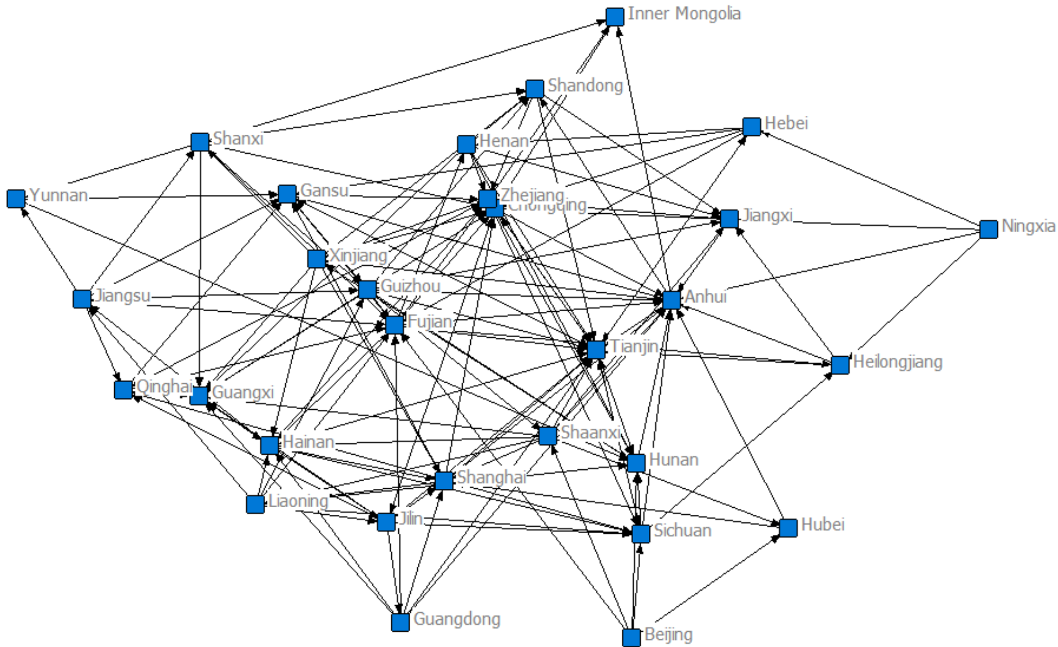
Carbon emission footprint spatial network in 2007
