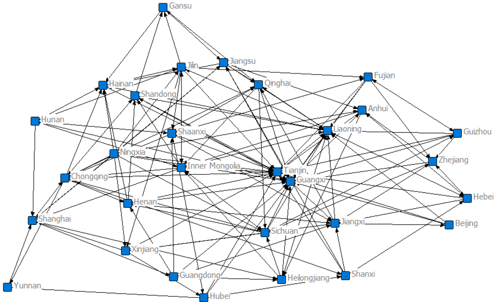
Carbon emission footprint spatial network in 2015
