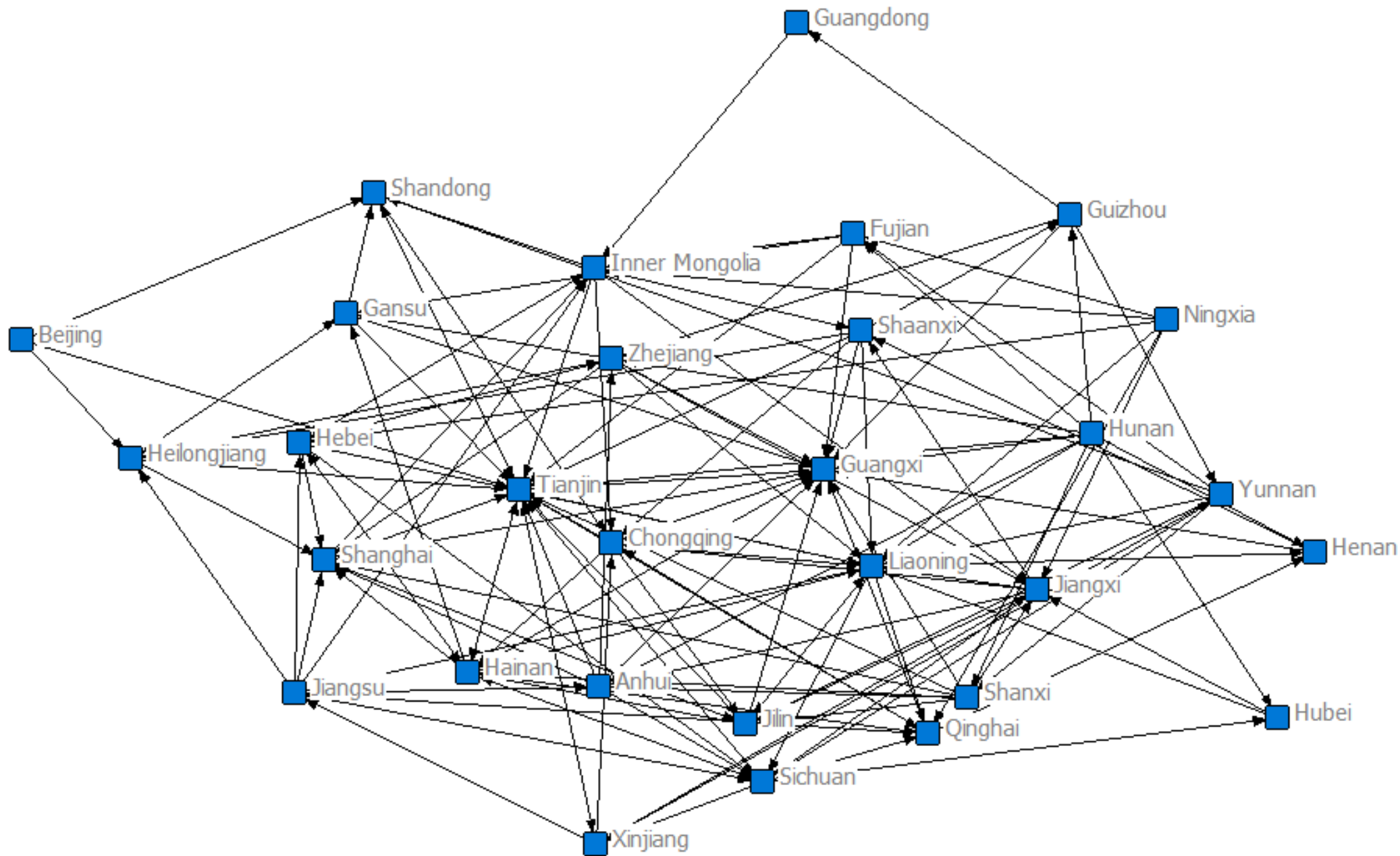
Carbon emission footprint spatial network in 2016
