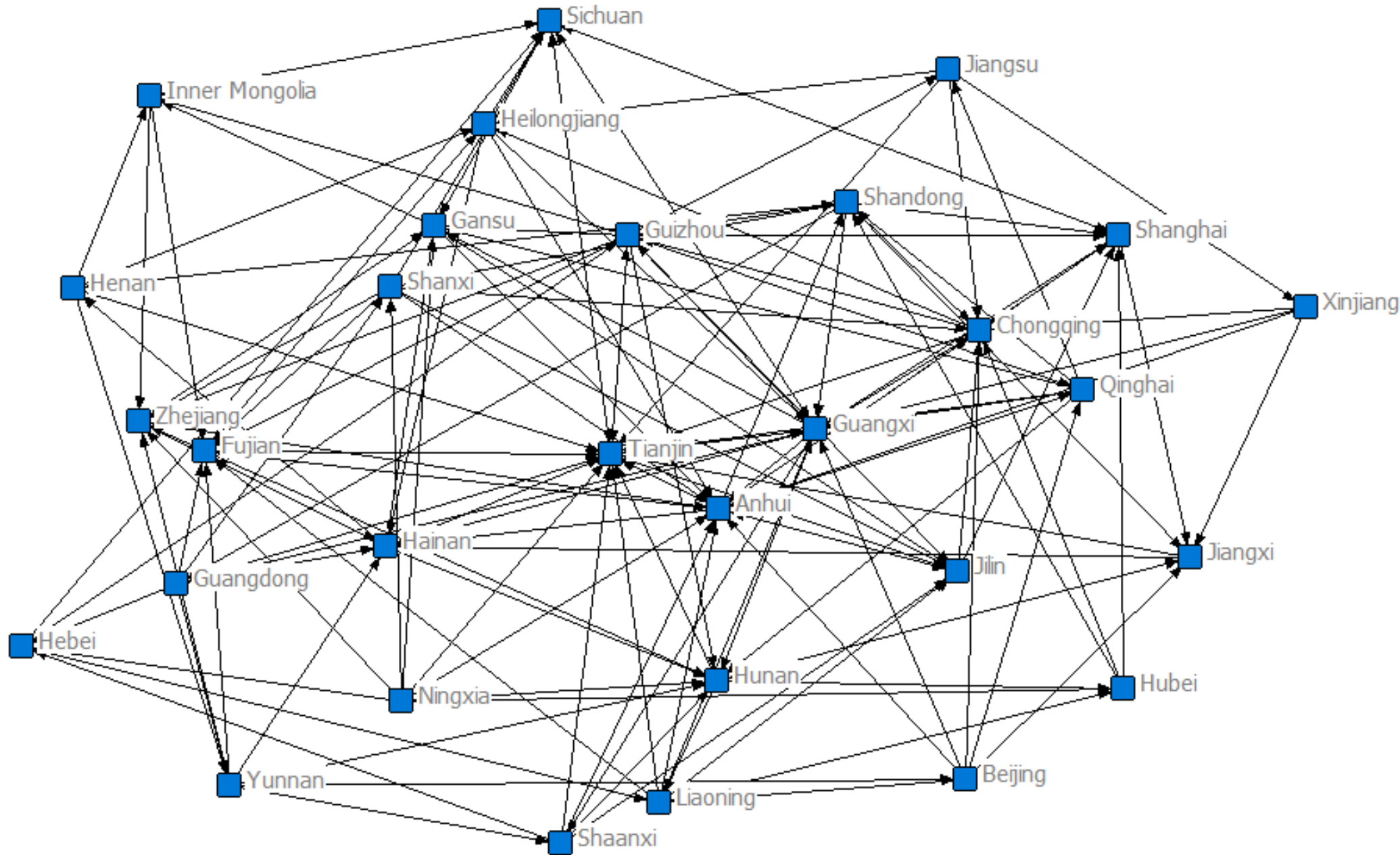
Carbon emission footprint spatial network in 2009
