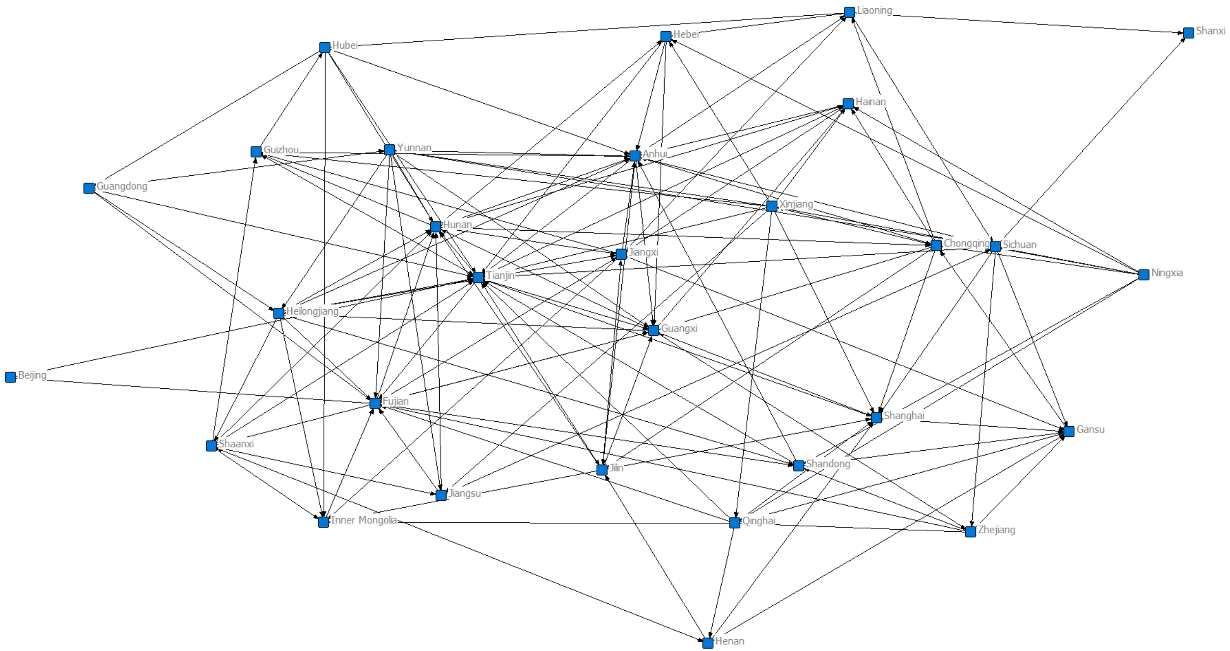
Carbon emission footprint spatial network in 2001
