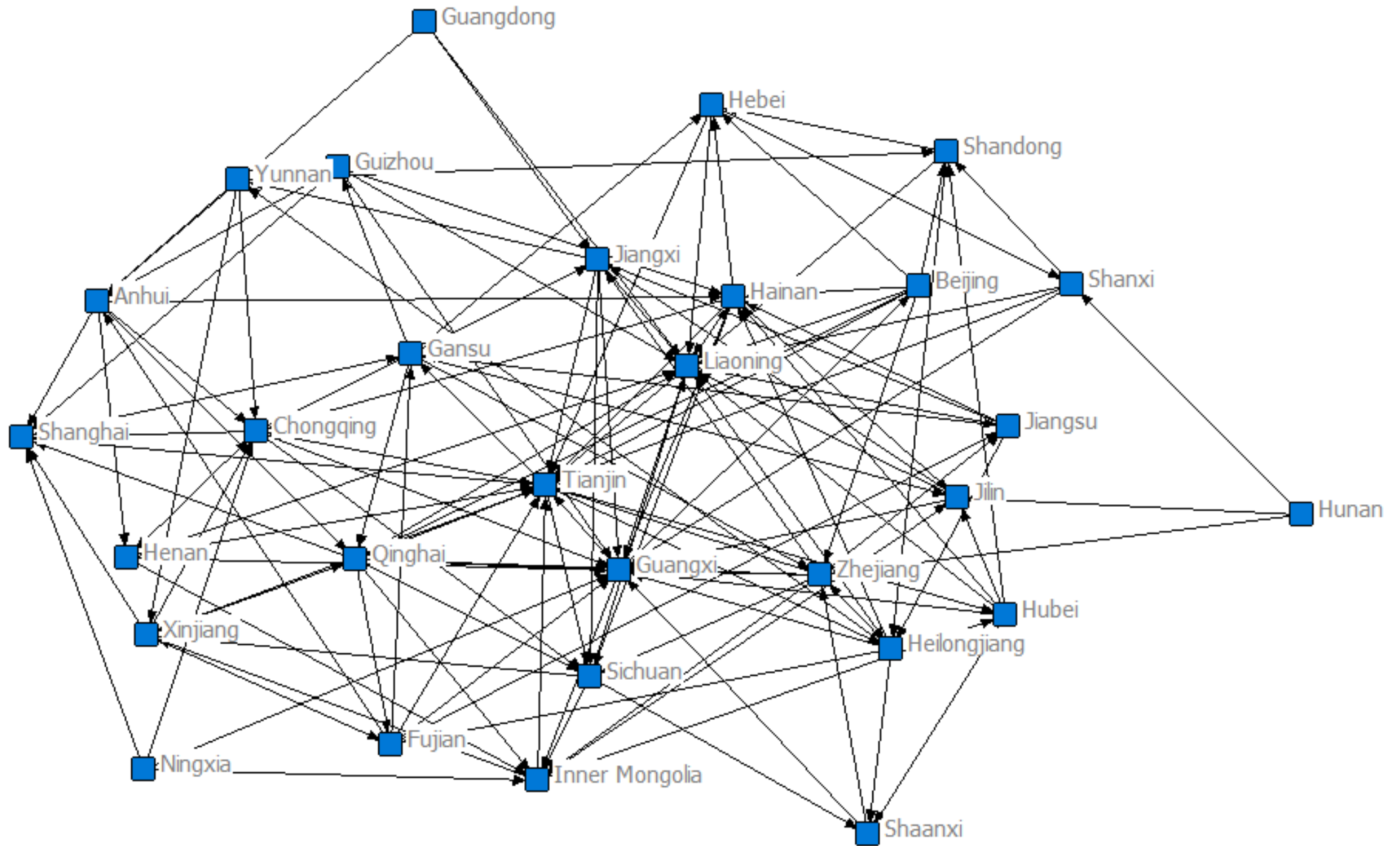
Carbon emission footprint spatial network in 2014
