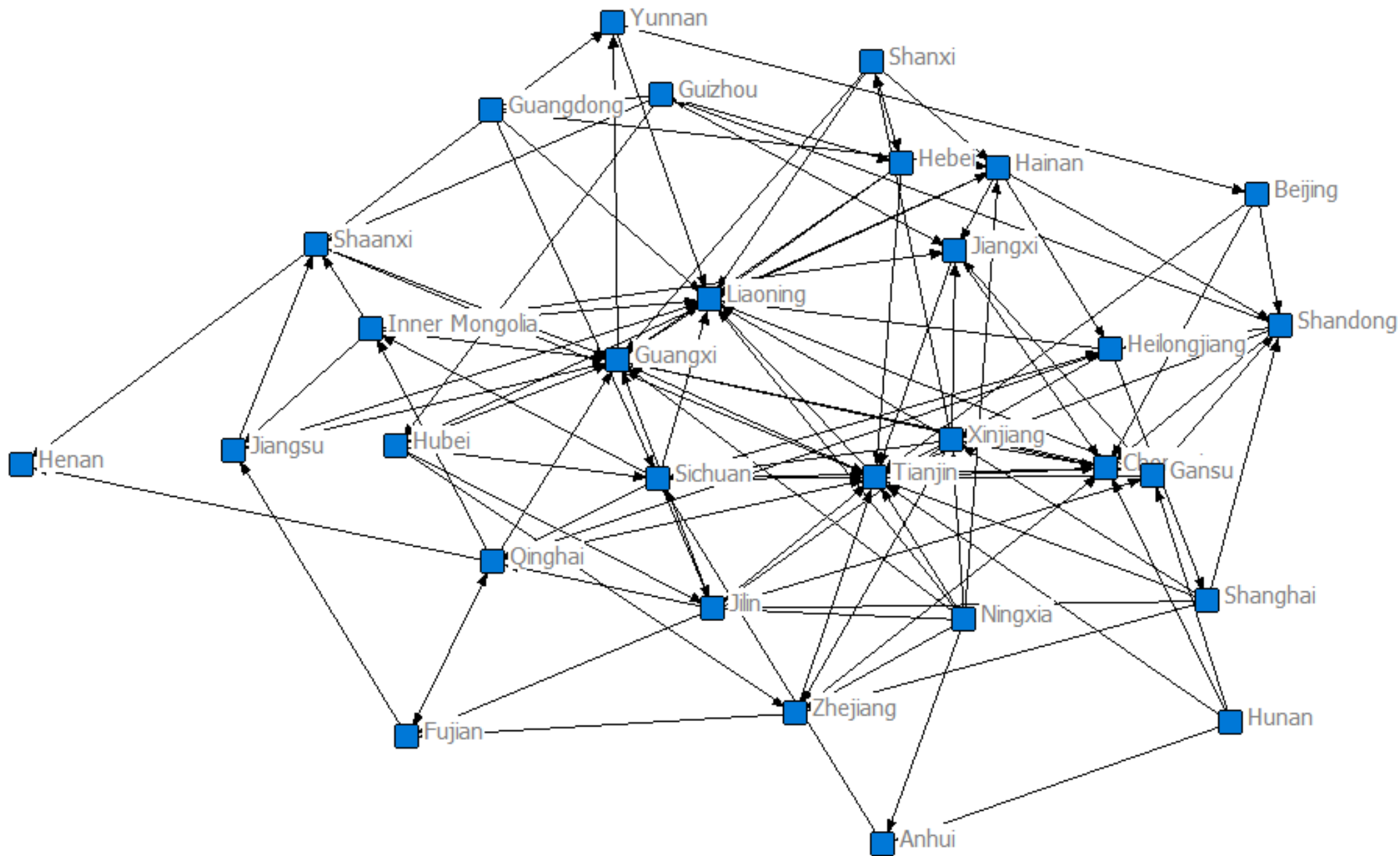
Carbon emission footprint spatial network in 2021
