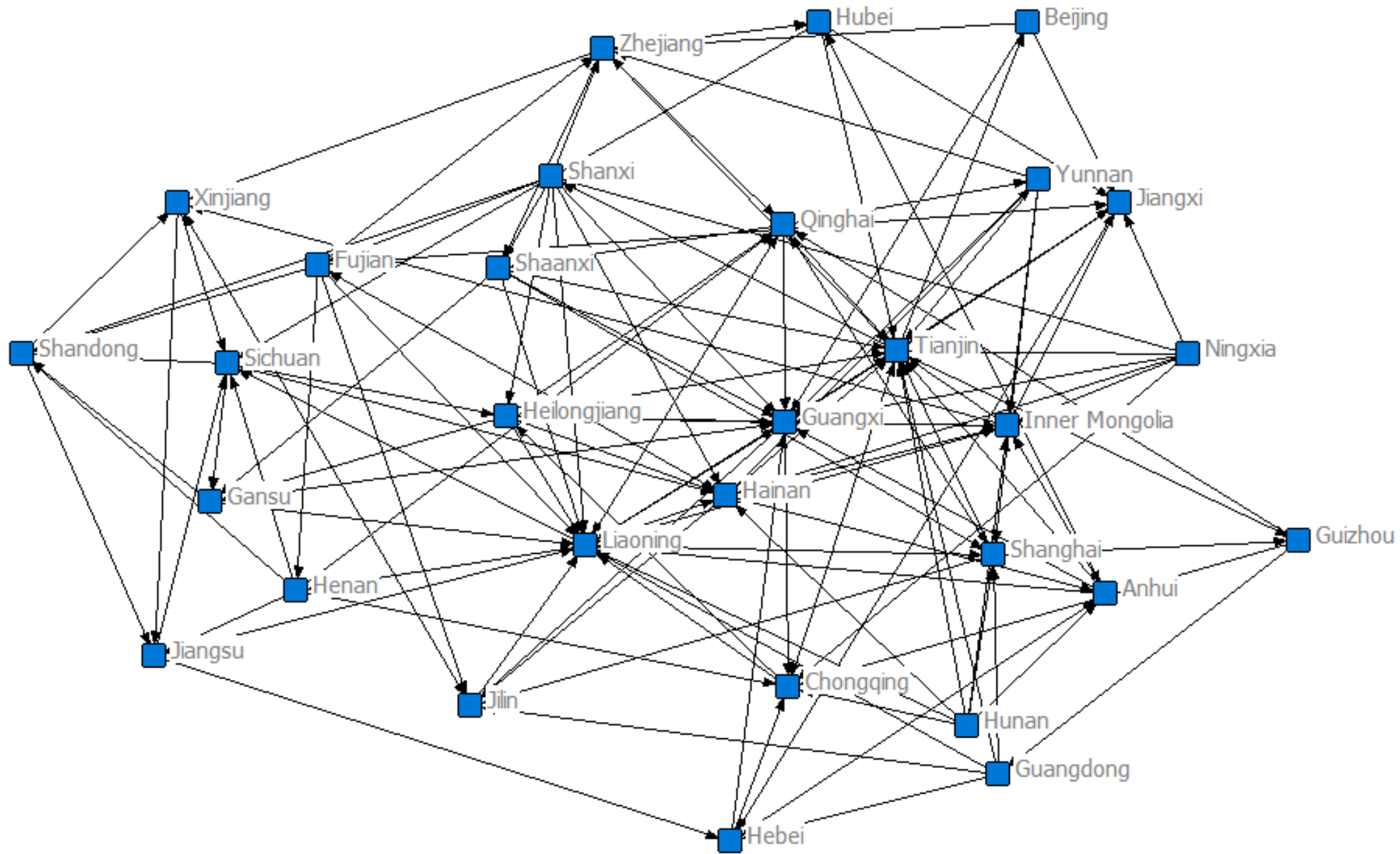
Carbon emission footprint spatial network in 2013
