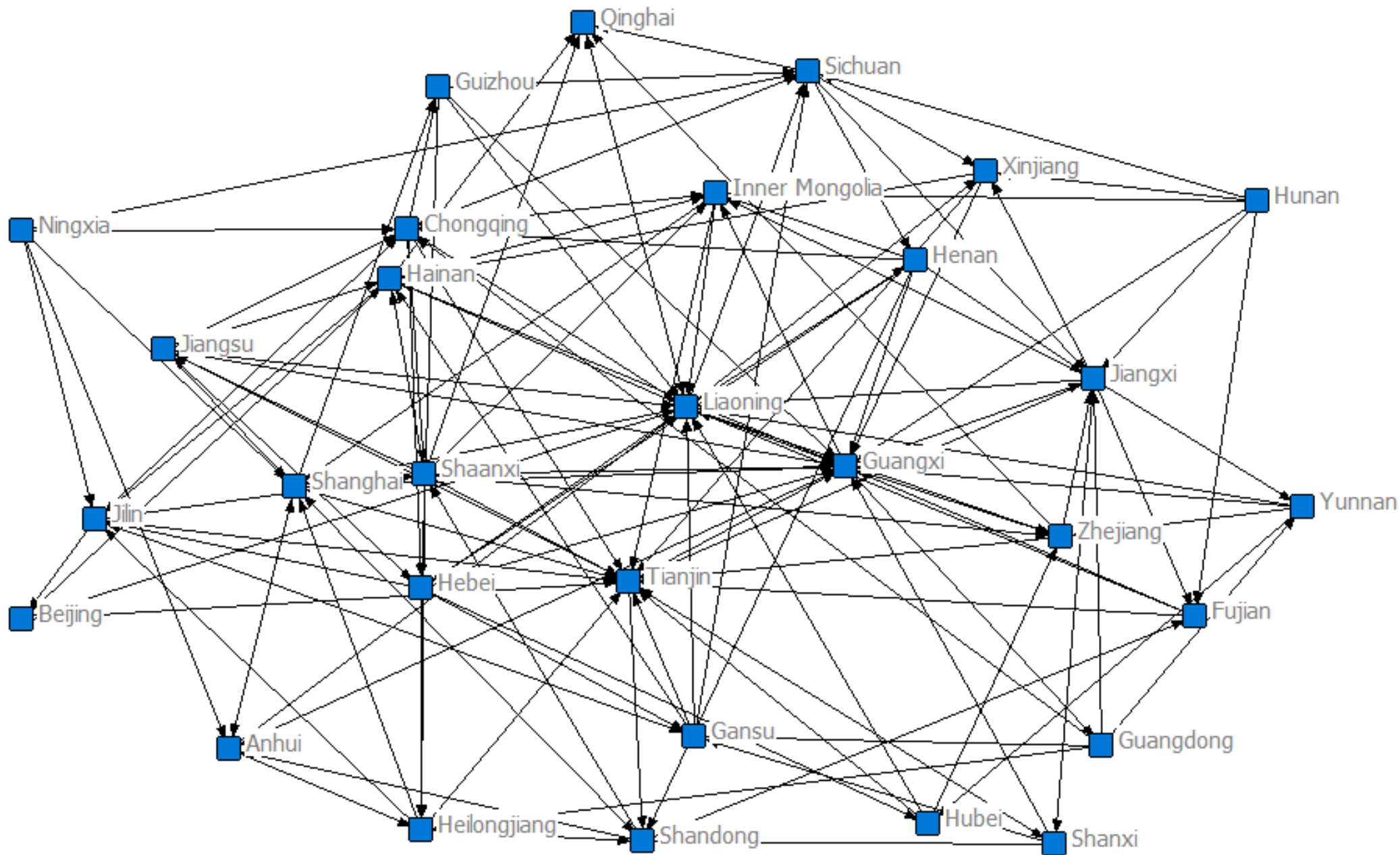
Carbon emission footprint spatial network in 2018
