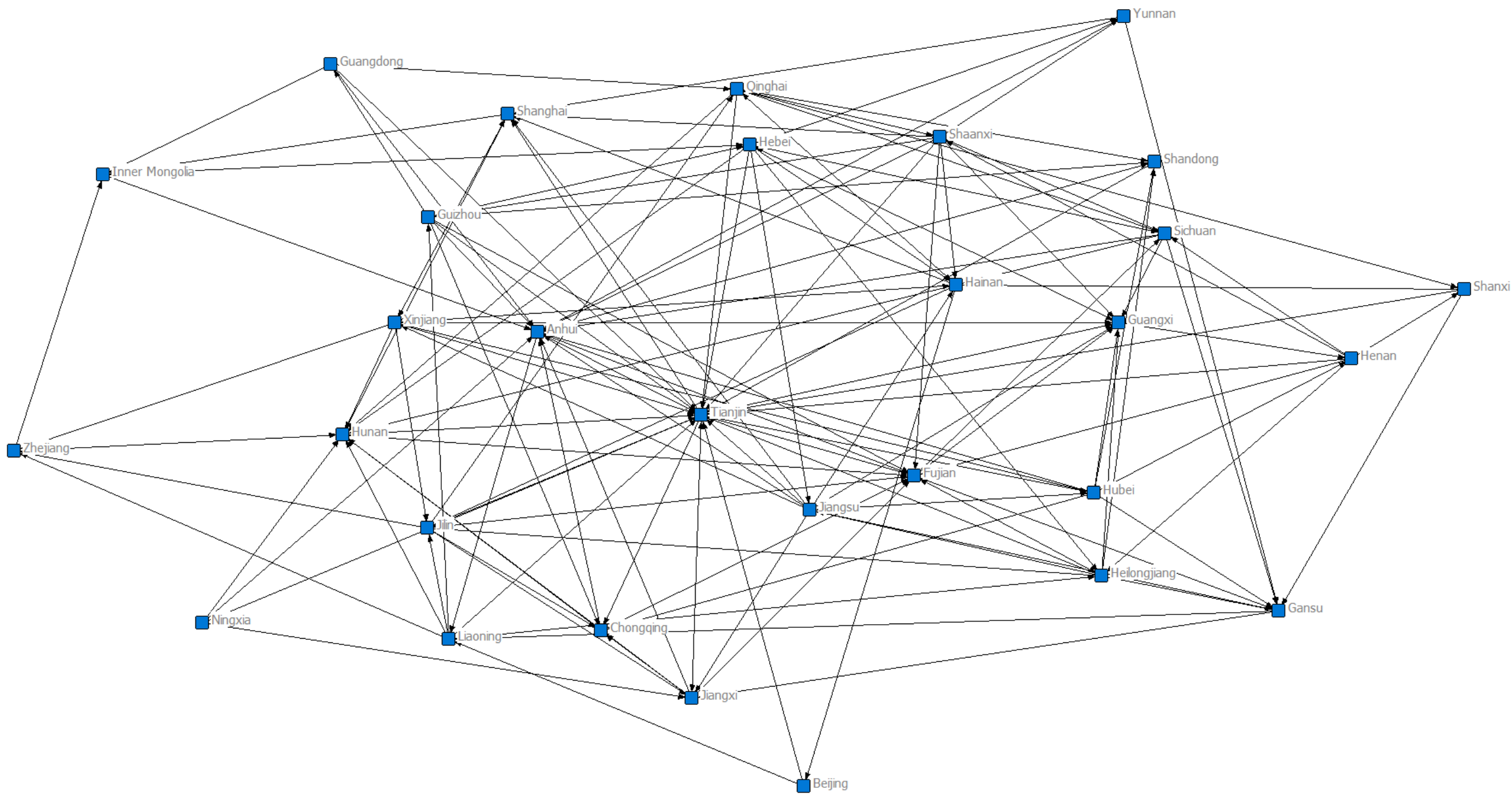
Carbon emission footprint spatial network in 2002
