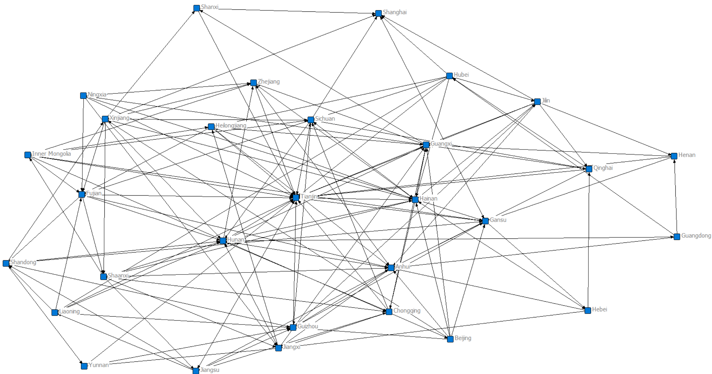
Carbon emission footprint spatial network in 2003
