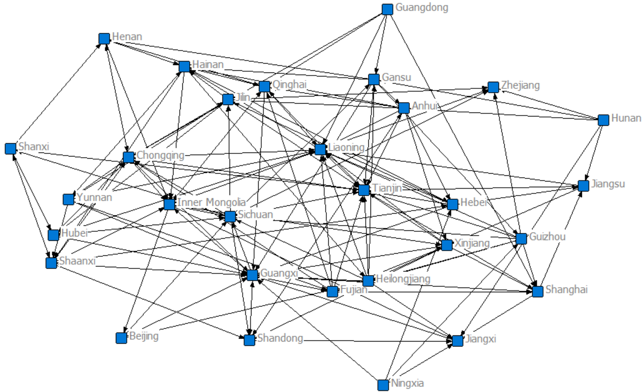
Carbon emission footprint spatial network in 2019
