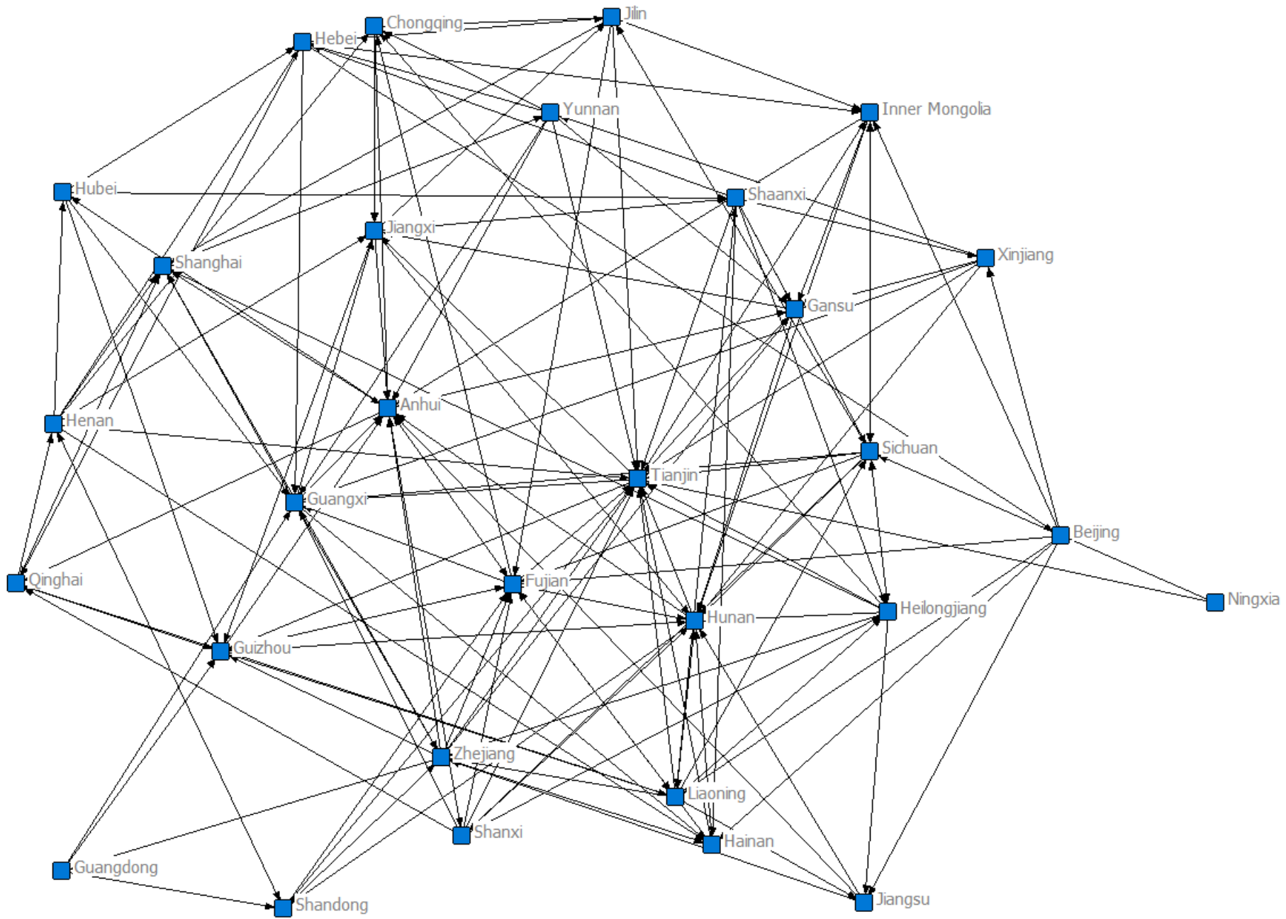
Carbon emission footprint spatial network in 2000
