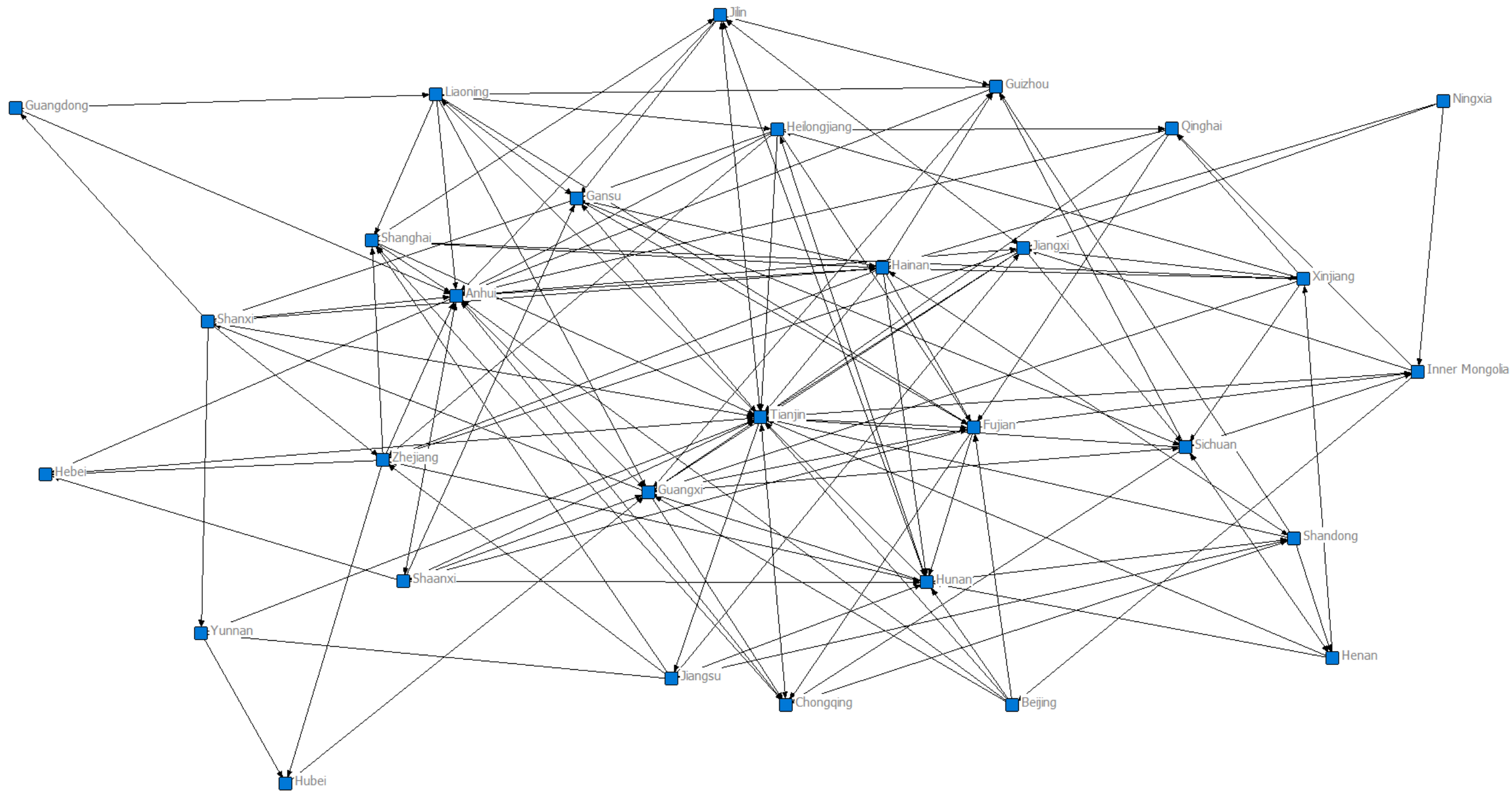
Carbon emission footprint spatial network in 2004
