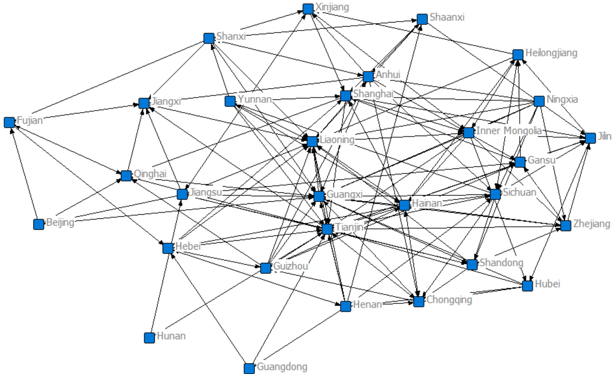
Carbon emission footprint spatial network in 2017
