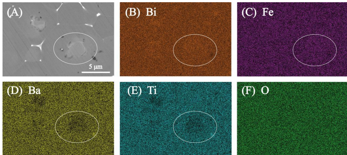
Figure S3. (A) BSE images of B_{1.03}F -BT ceramic and EDS elemental mapping results (B) Bi, (C) Fe, (D) Ba, (E) Ti and (F) O.
