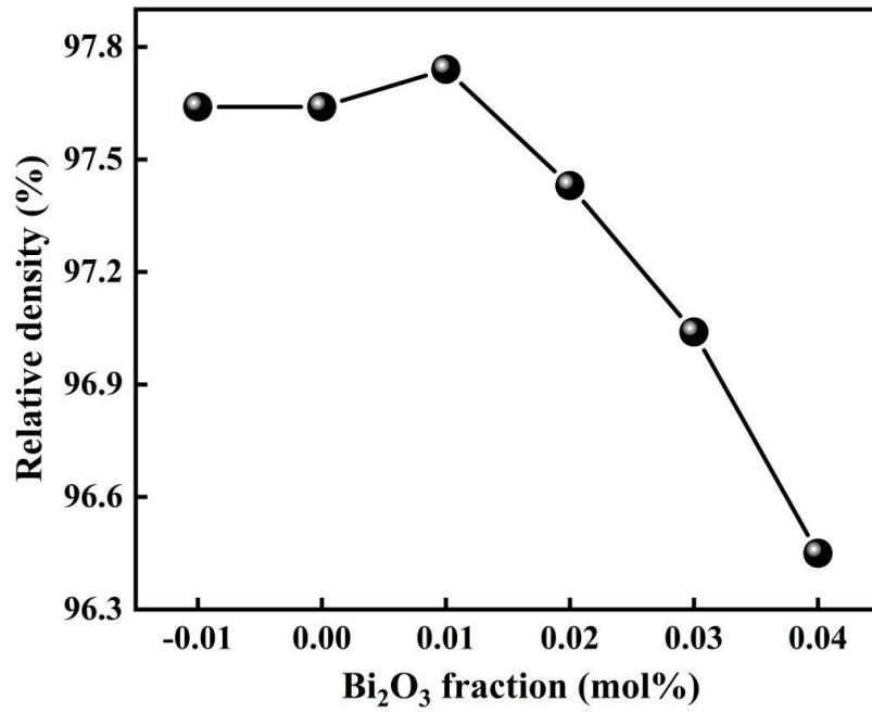
Figure S1. The densities of the B_{1+x}F -BT ceramics.
