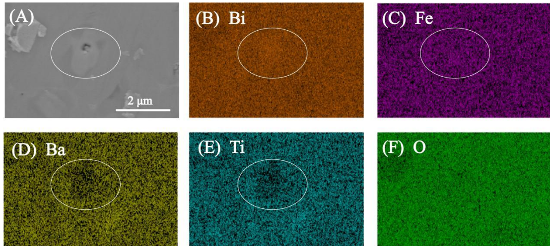
Figure S2. (A) BSE images of B_{0.99}F -BT ceramic and EDS elemental mapping results (B) Bi, (C) Fe, (D) Ba, (E) Ti and (F) O.
