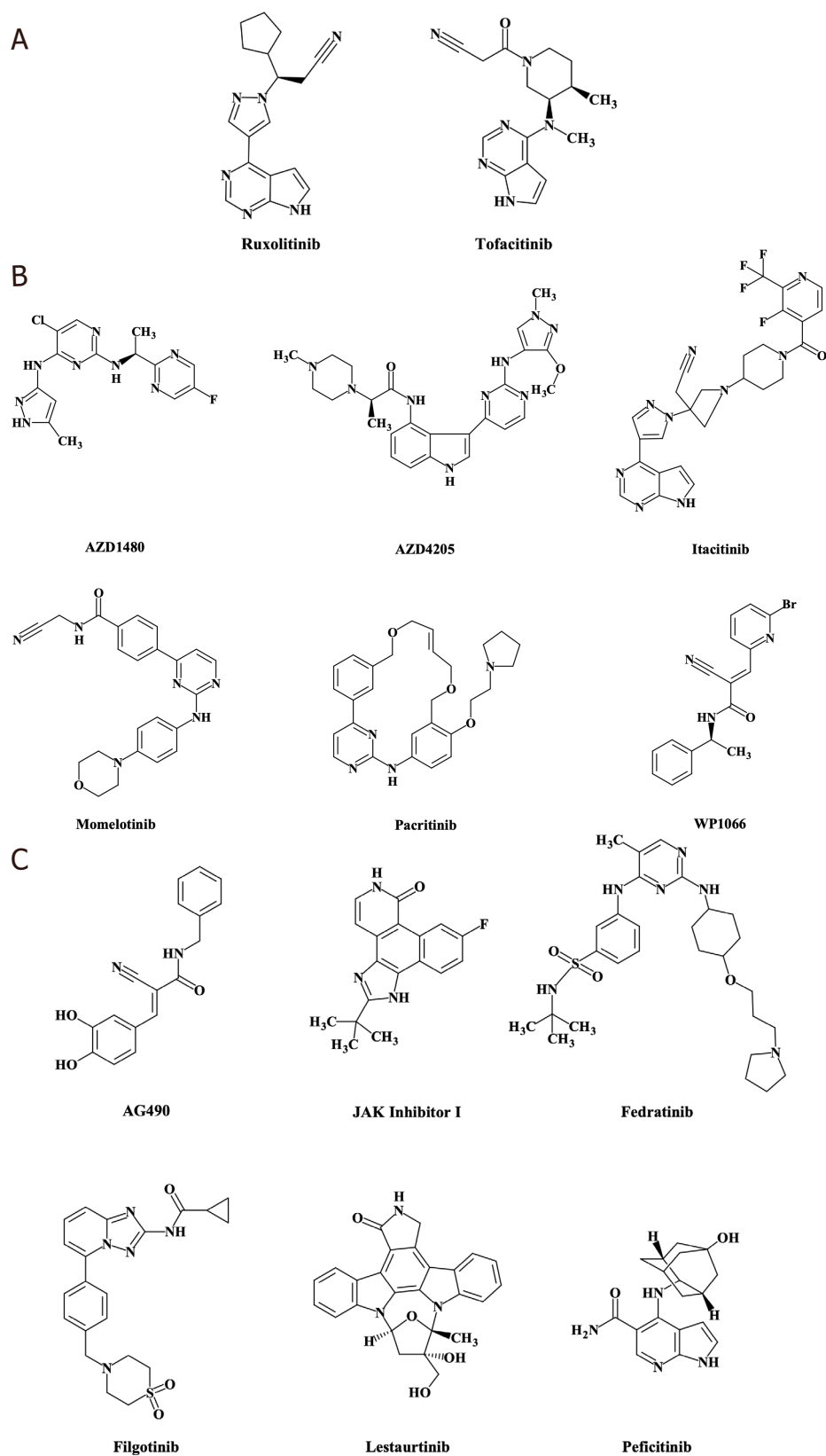
Figure 2. JAK inhibitors: chemical structures for JAK inhibitors described in this review were created using MarvinSketch software downloaded from ChemAxon (Budapest, Hungary) [115,171-183] . Food and Drug Administration (FDA)-approved JAK inhibitors that have been tested clinically in solid tumors (A); JAK inhibitors that are not FDA approved but have been tested clinically in solid tumors (B); JAK inhibitors that have only been tested in solid tumor preclinical models, and lestaurtinib, which has been tested clinically in solid tumors for its activity against other targets (C). Structures for INCB047986 and INCB052793 are not publicly available and therefore are not shown in this figure. *FDA approved for another indication; JAKs: Janus kinases
